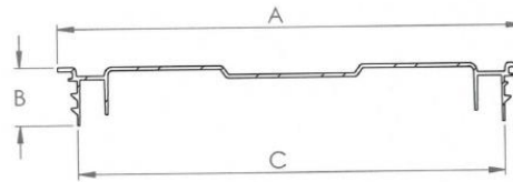
SECTION C-C SCALE 1 : 3
